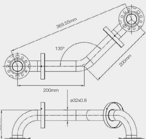
450MM ANGLED GRAB BAR - 32MM Ø DIAMETER
