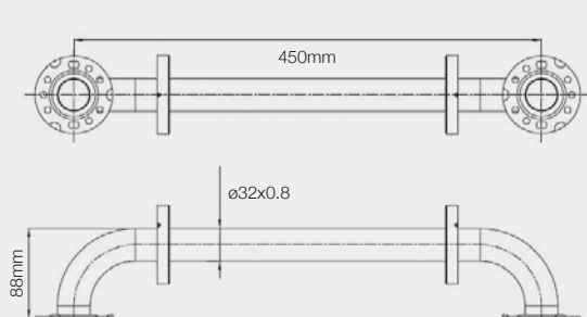
450MM GRAB BAR - 32MM Ø DIAMETER
