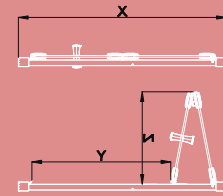
BIFOLD - DOOR OPEN POSITION MEASUREMENTS
