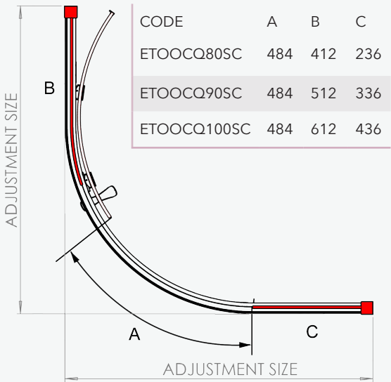
MAGNETIC CUSHION CLOSE DOOR SYSTEM
