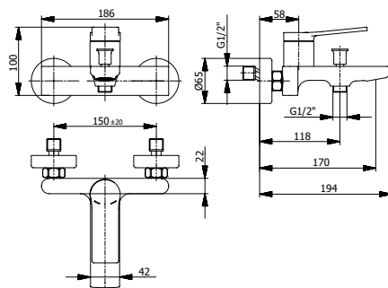
Operating Pressure Min: 1 bar | Max: 5 bar
