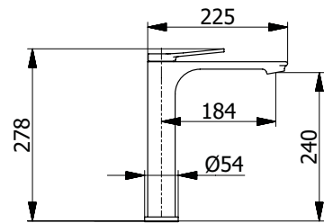
Operating Pressure Min: 1 bar | Max: 5 bar
