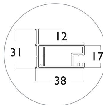
PROFILE (identical on both ends)
