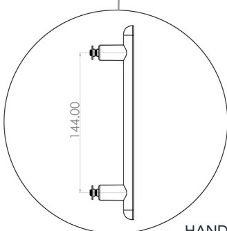
HANDLE
